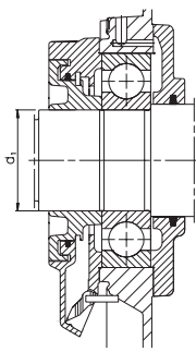
Labyrinth seal
